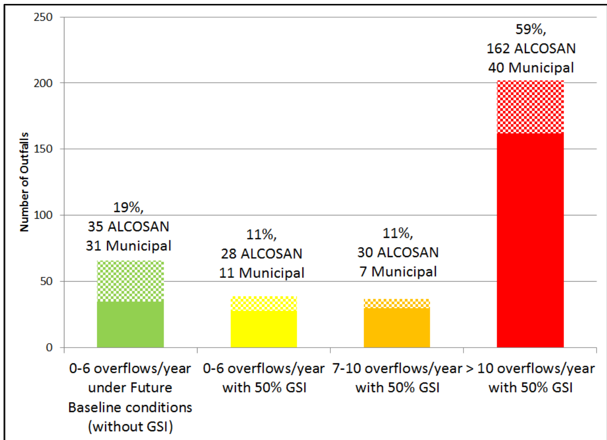
Figure 10-25: Count of outfalls in various Overflow Frequency ranges for the GSI only Alternative
