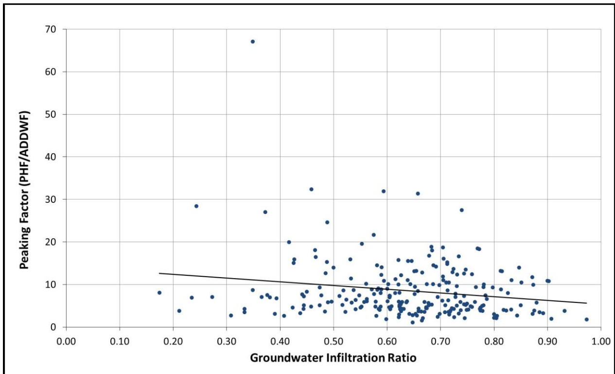
Figure 10-14: Relationship between Wet Weather Peaking Factor and Groundwater Infiltration in the ALCOSAN Service Area
