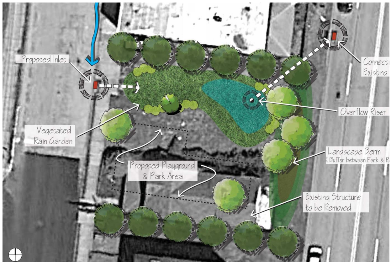
Figure 10-60: East Pittsburgh GSI Concept Plan
