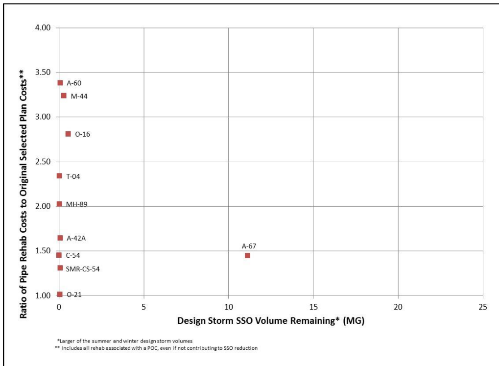
Figure 10-31: Potential of I/I Reduction to Eliminate SSOs – Point of Connection Sewersheds– Cost Ratio of One or More
