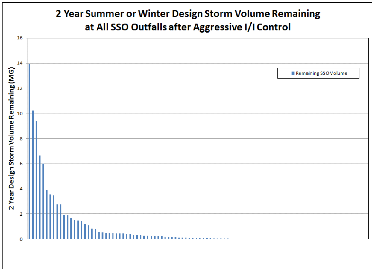
Figure 10-33: Remaining SSO Volume After Aggressive I/I Reduction
