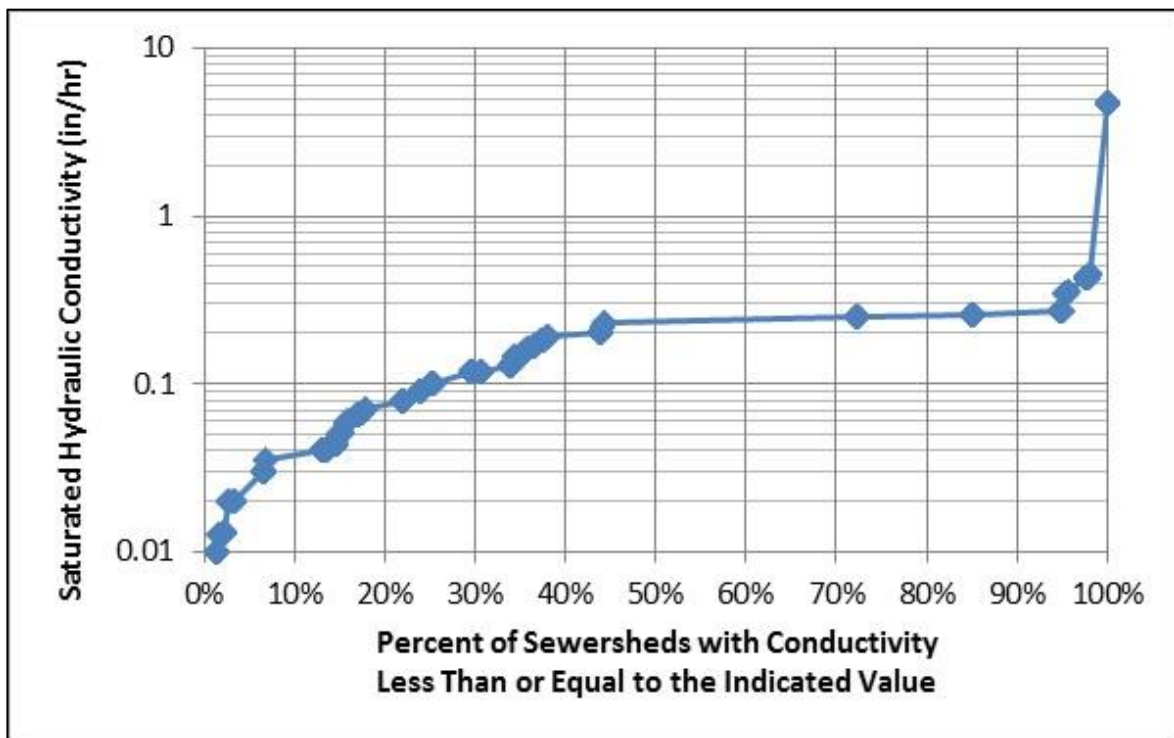
Figure 10-6: Cumulative Distribution of Saturated Vertical Hydraulic Conductivity Assumptions in Hydrologic Models used in the WWP
