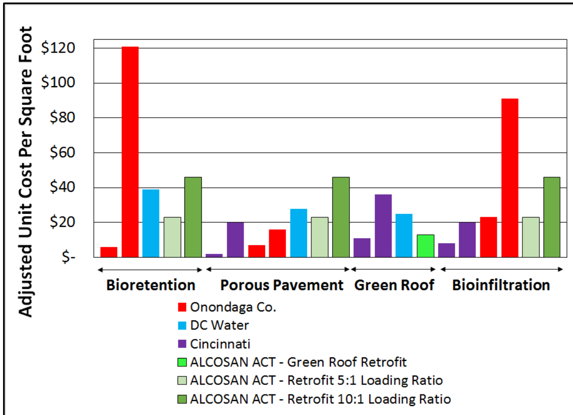
Figure 10-10: National Comparison – Construction Cost ($ per Square Foot) of Installed GSI
