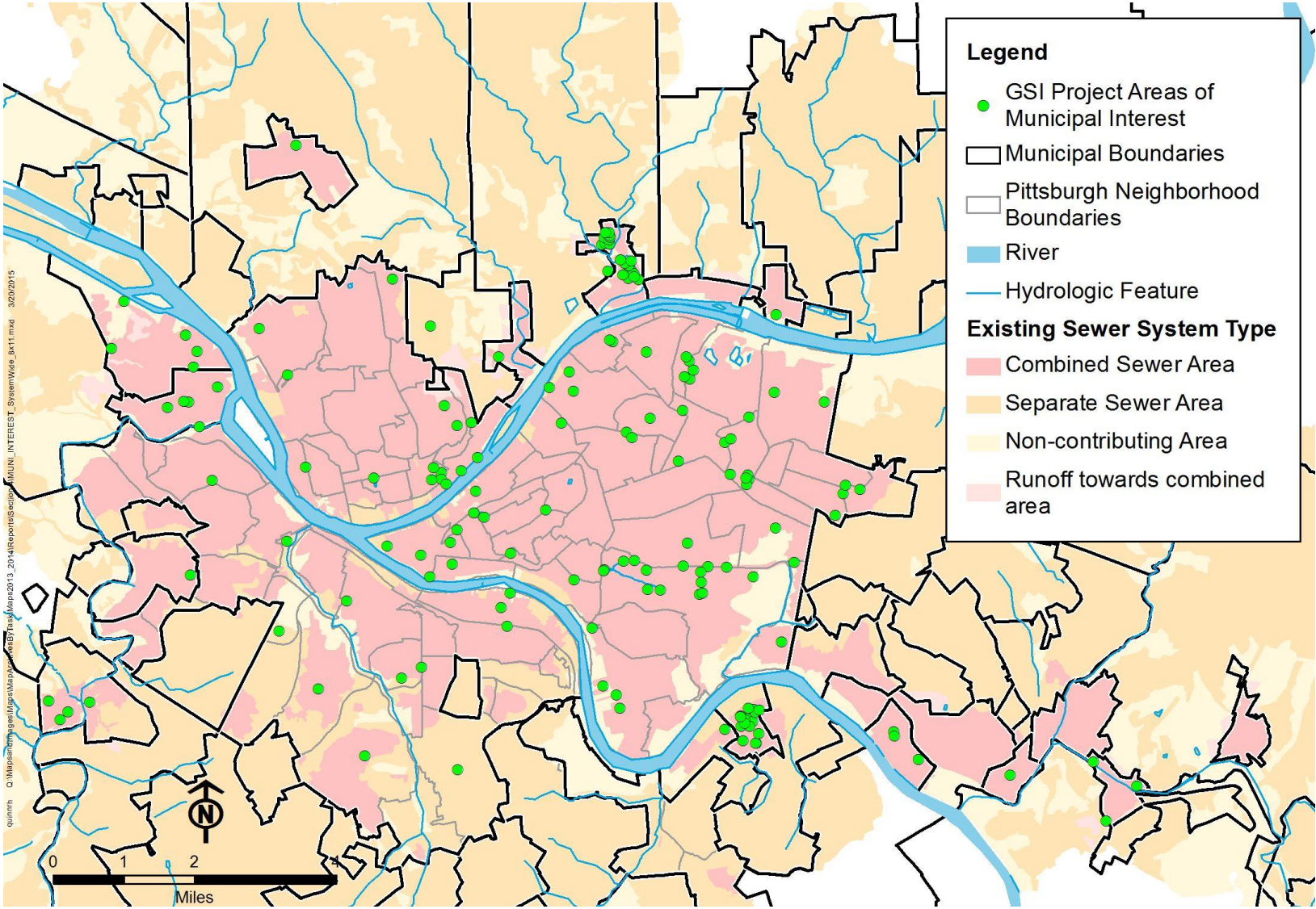
Figure 10-46: Municipal and Stakeholder Identified GSI Projects
