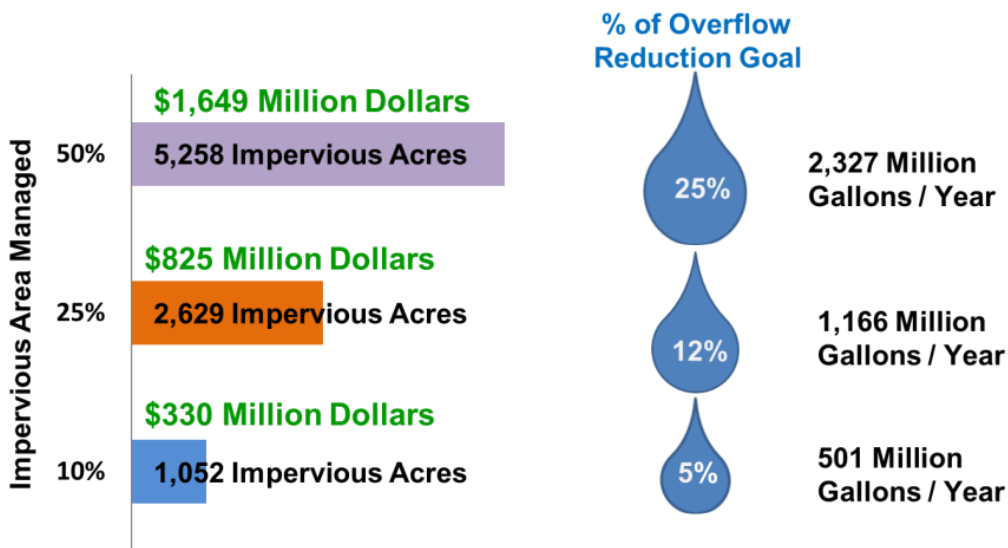
Figure 10-16: Capital Cost and Overflow Reduction Benefit of Green Stormwater Infrastructure (Simulations 1, 2, 3)
