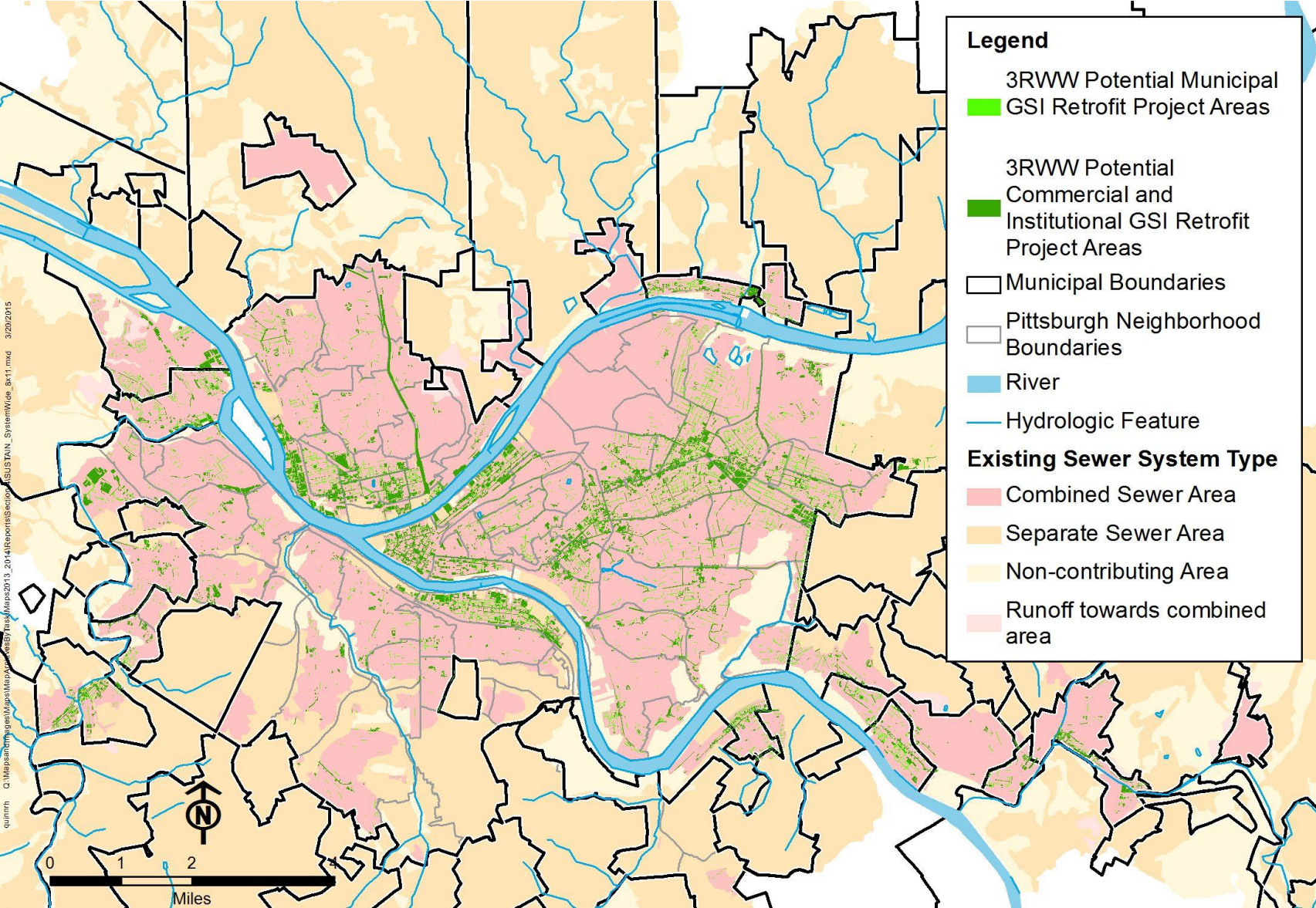
Figure 10-38: Potential Green Stormwater Infrastructure Municipal Retrofit Project Locations identified by 3RWW
