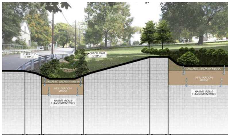
Figure 10-2: ALCOSAN Design Rendering for McKinley Park in the Beltzhoover Neighborhood of Pittsburgh
