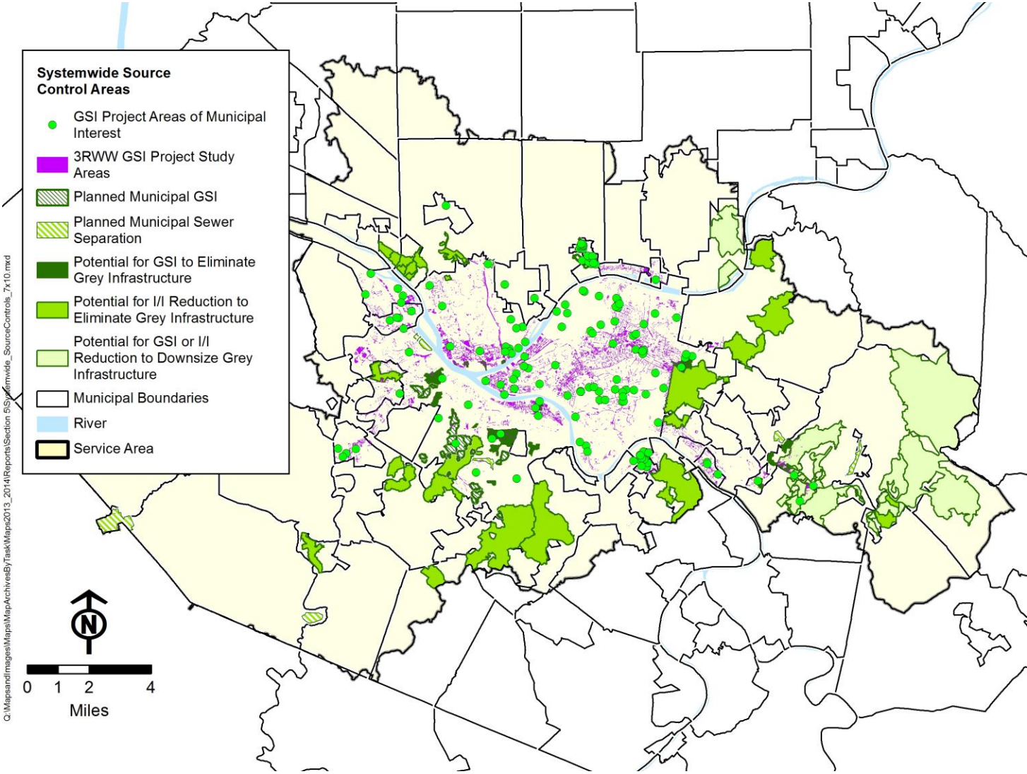
Figure 10-66: Areas of Identified Project Opportunities
