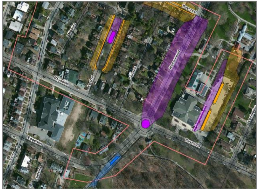
Figure 10-43: Layout of Conceptual GSI Projects in Frick Museum Area, Point Breeze
