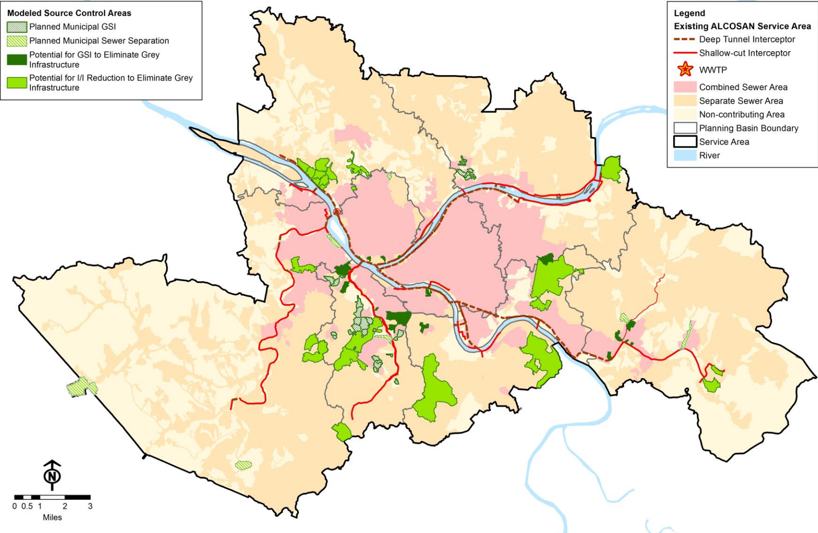
Figure 10-67: Source Control Areas Included in Greener Alternative
