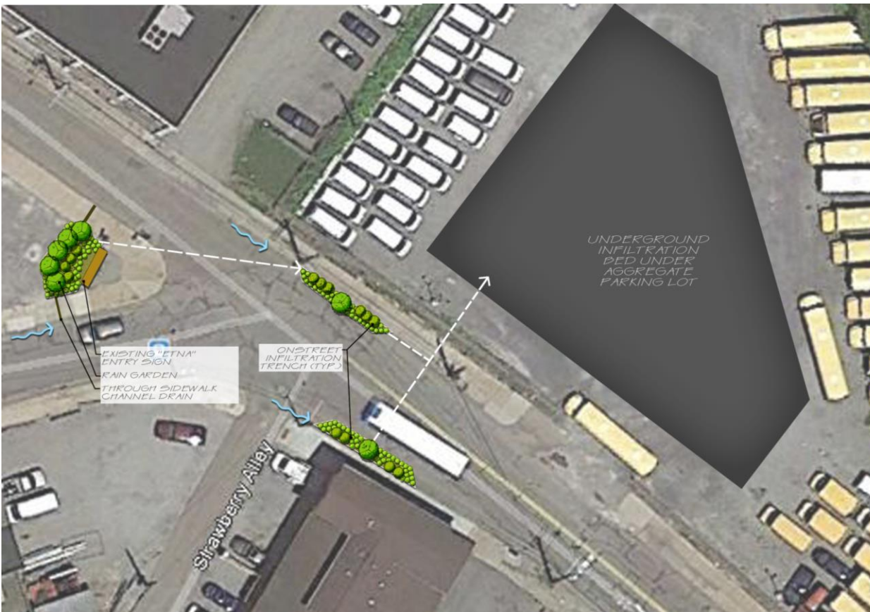
Figure 10-57: Etna Borough GSI Concept Plan
