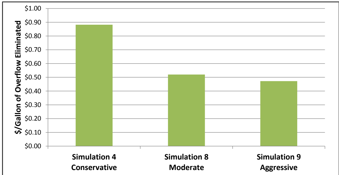
Figure 10-20: Range in Cost-Effectiveness for Simulations 4, 8, and 9
