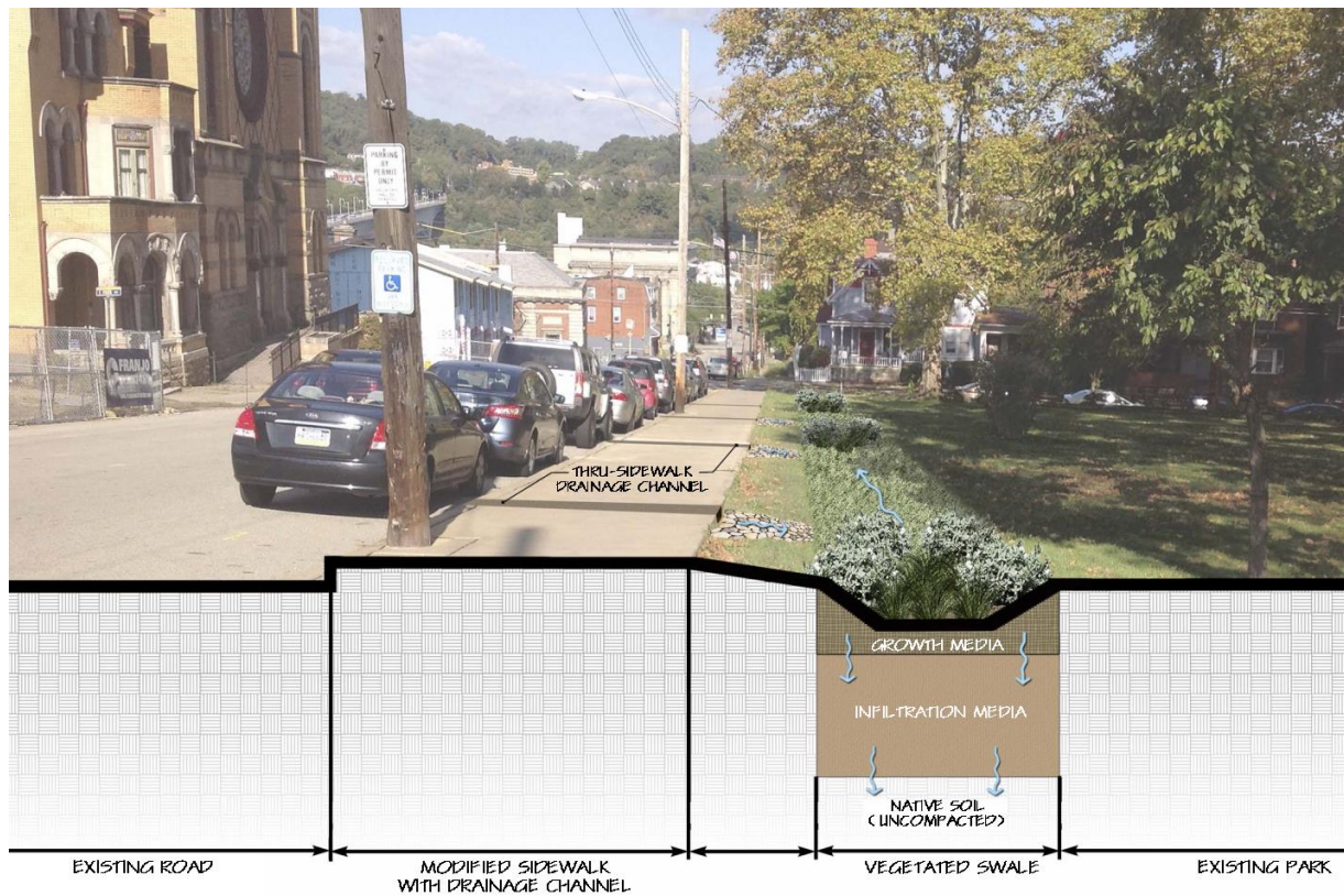
Figure 10-52: Homestead Borough Frick Park GSI Cross-Sectional Rendering
