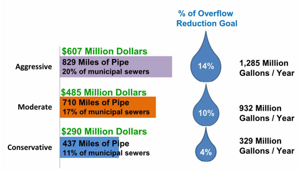
Figure 10-19: Capital Cost and Overflow Reduction Benefit of I/I Reduction (Simulations 4, 8, 9)
