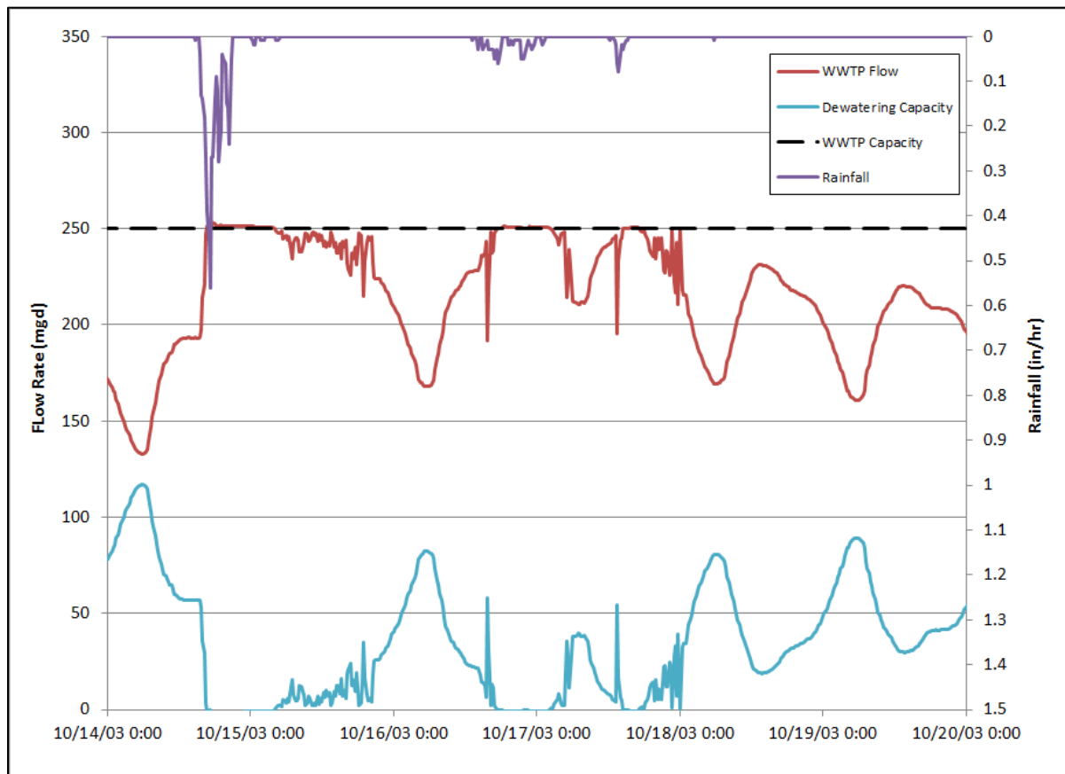
Figure 10-4: Example of System Wet Weather Treatment and Dewatering Capacity
