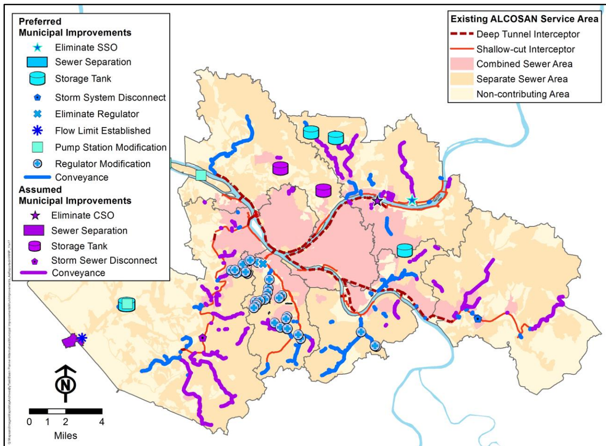
Figure 10-24: Preferred and Assumed Municipal Improvements as Reflected in ALCOSAN’s WWP (August 2012)
