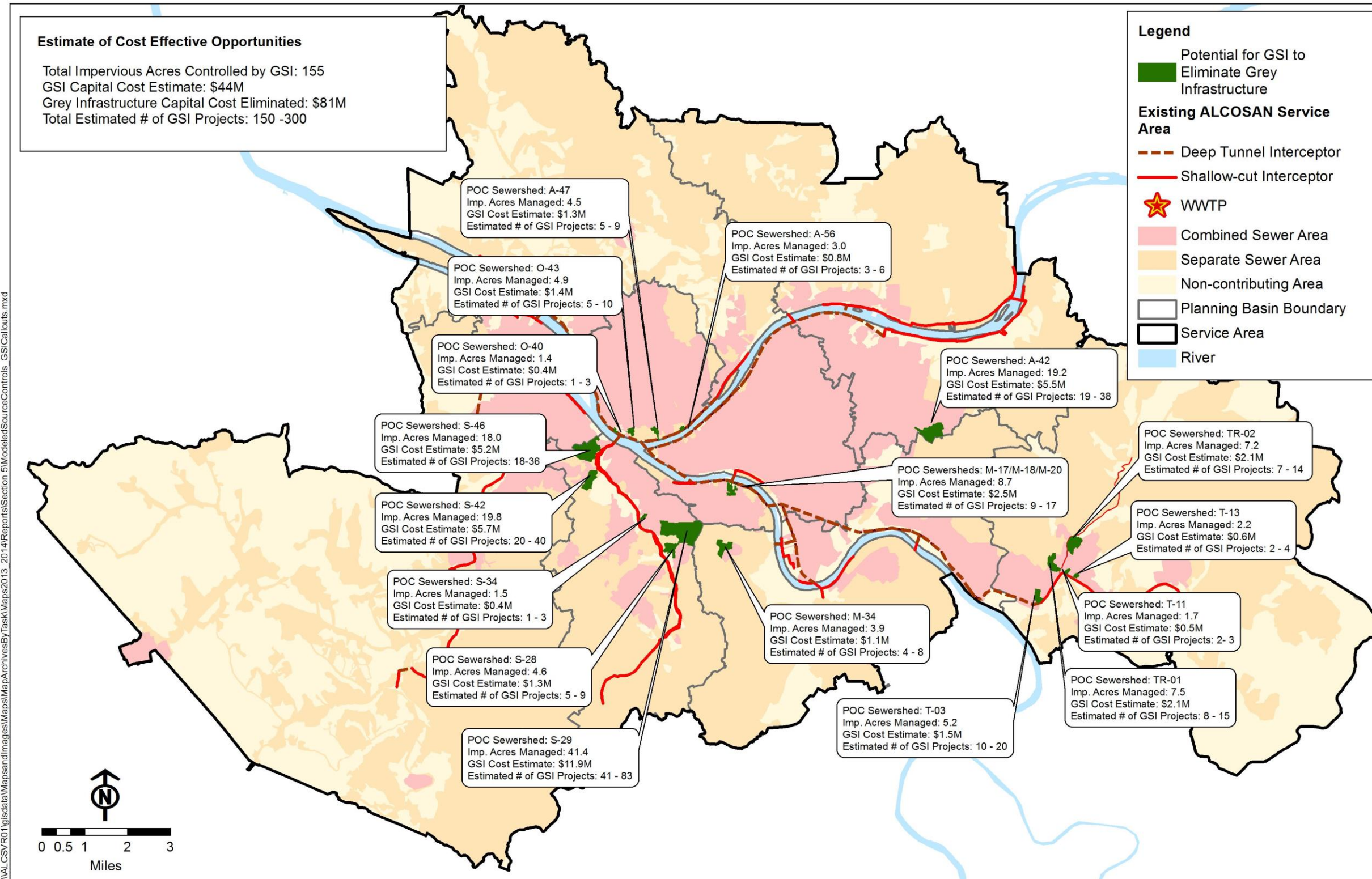
Figure 10-68: GSI Opportunities Included in Greener Alternative
