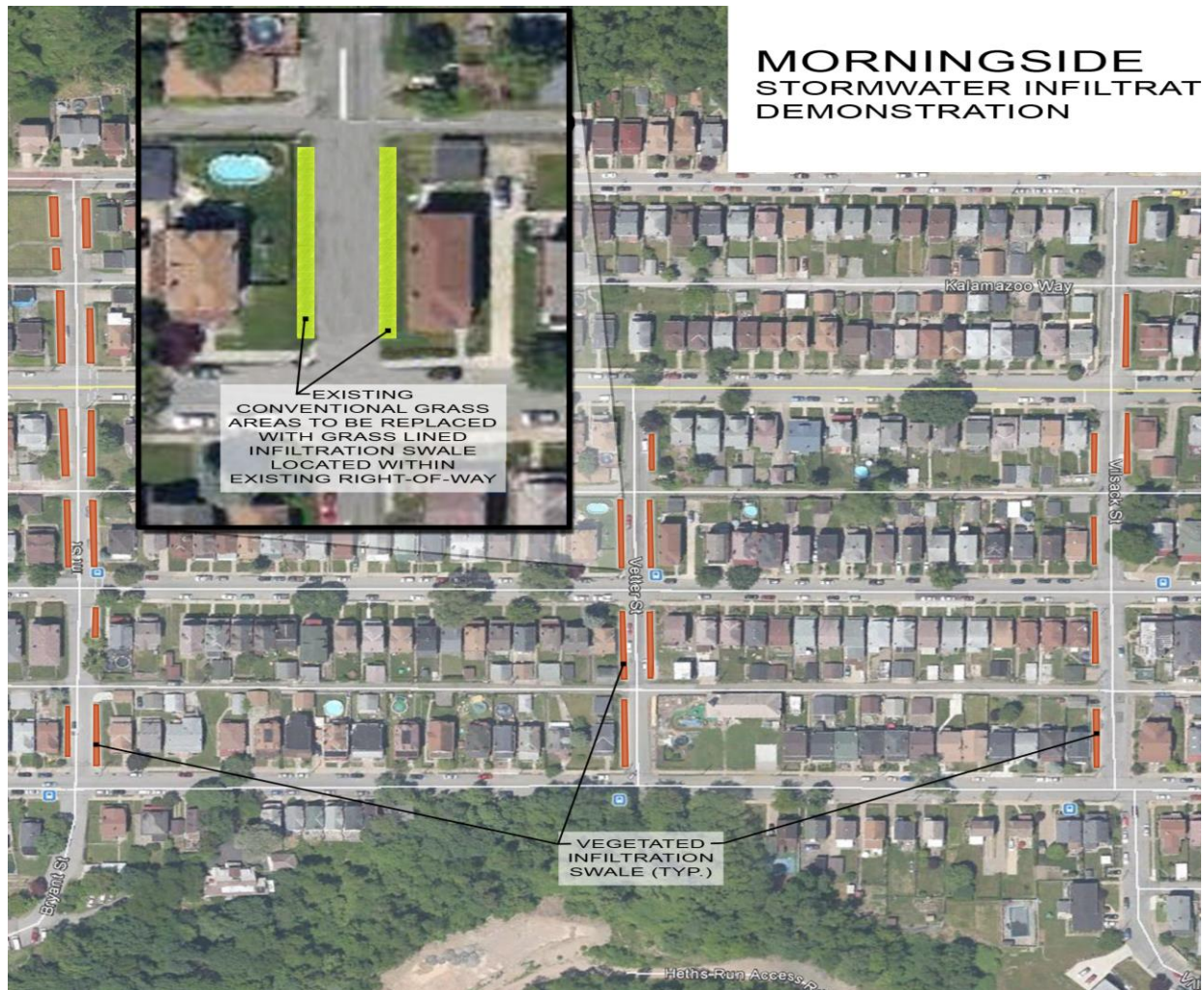
Figure 10-59: Morningside GSI Concept Plan
