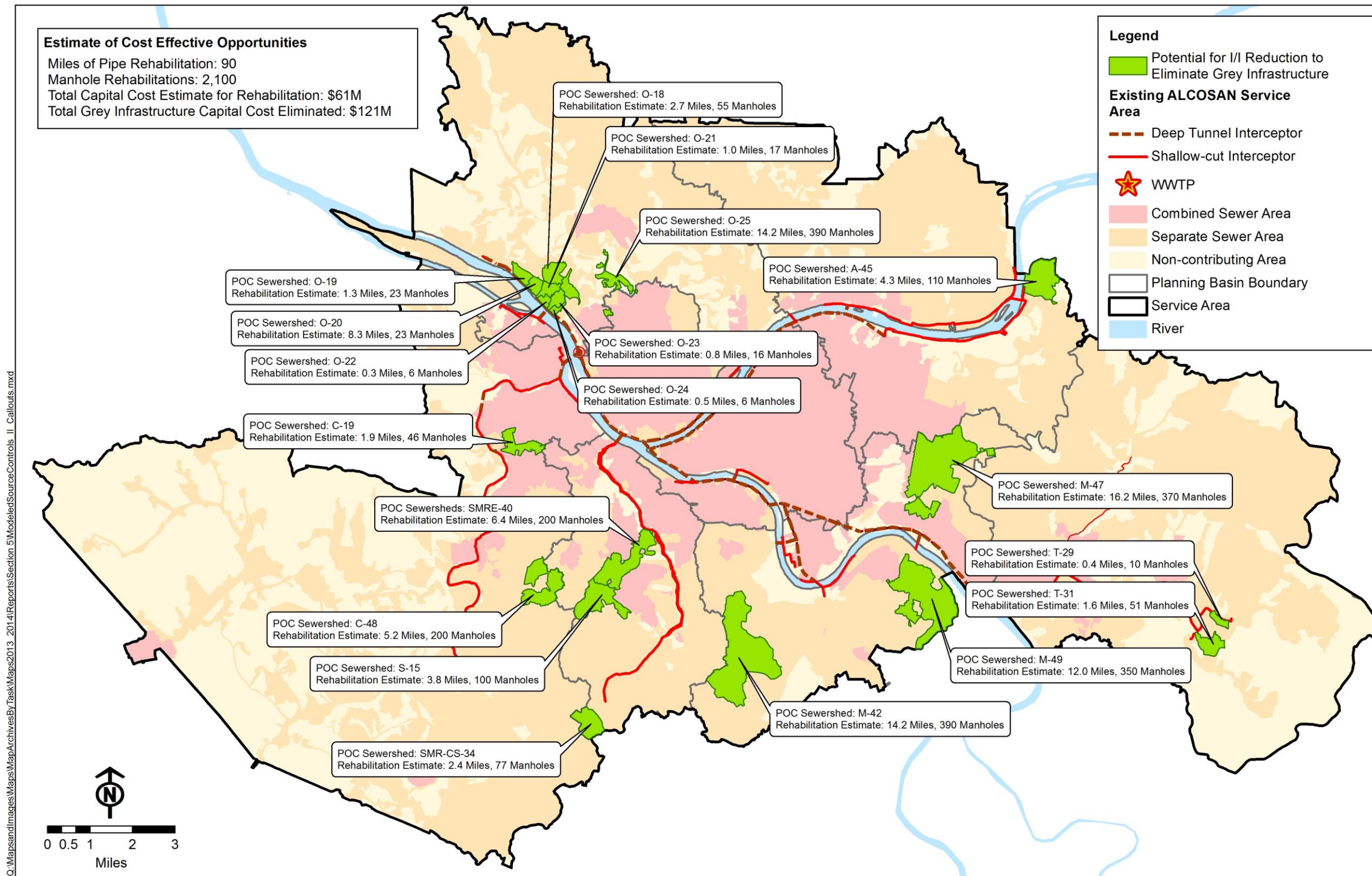
Figure 10-69: I/I Reduction Opportunities Included in Greener Alternative
