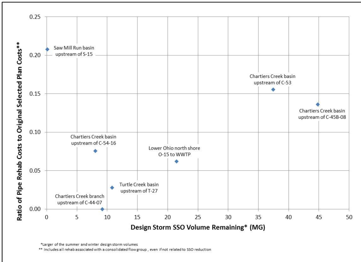
Figure 10-29: Potential of I/I Reduction to Eliminate SSOs – Groups of Points of Connections
