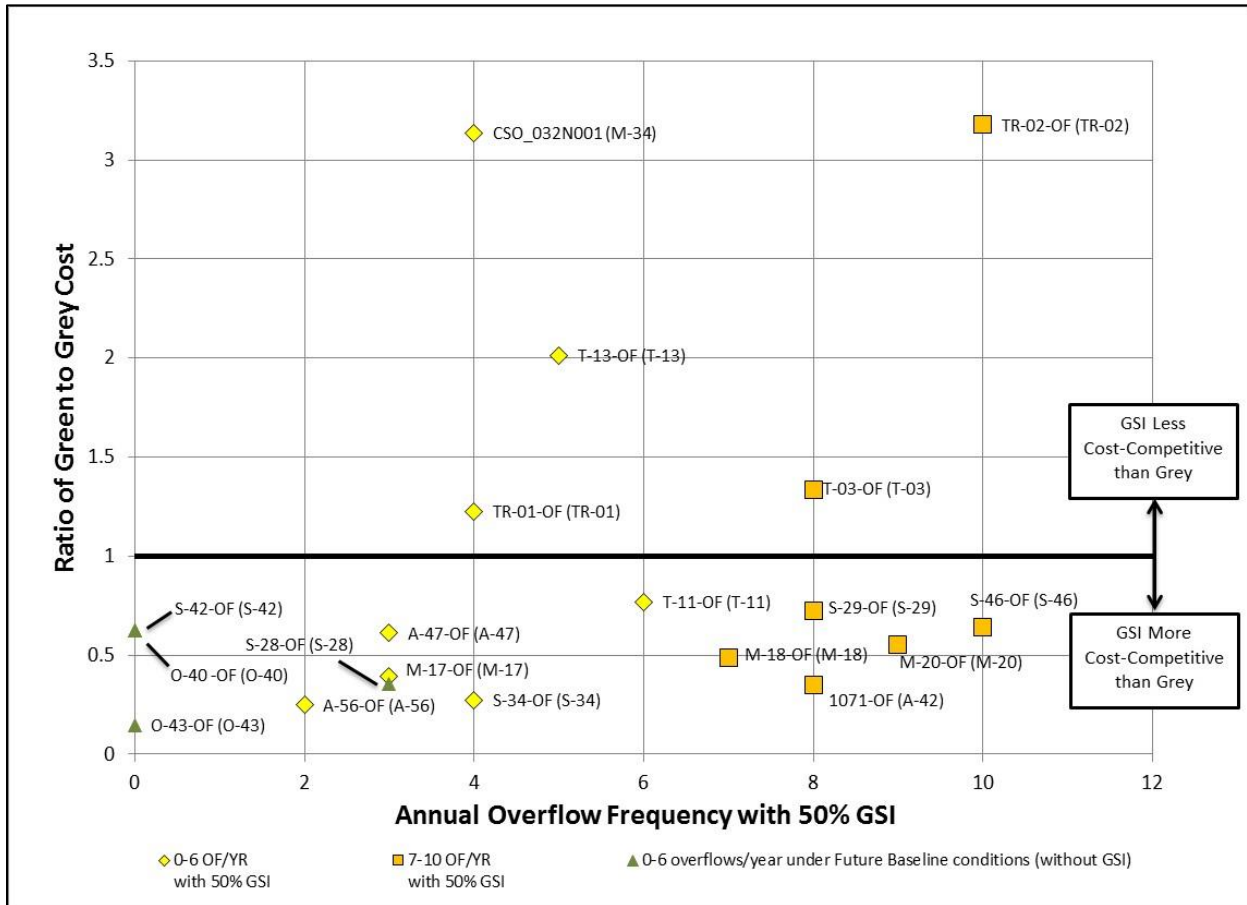
Figure 10-28: Cost Comparison Results for 19 Outfalls Analyzed with 50% of Impervious Cover Managed with GSI
