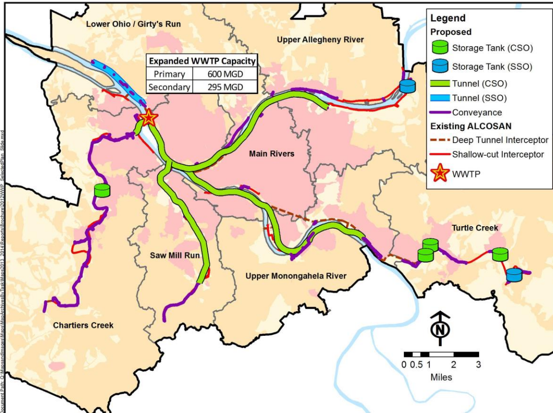
Figure 10-34: Selected Plan
