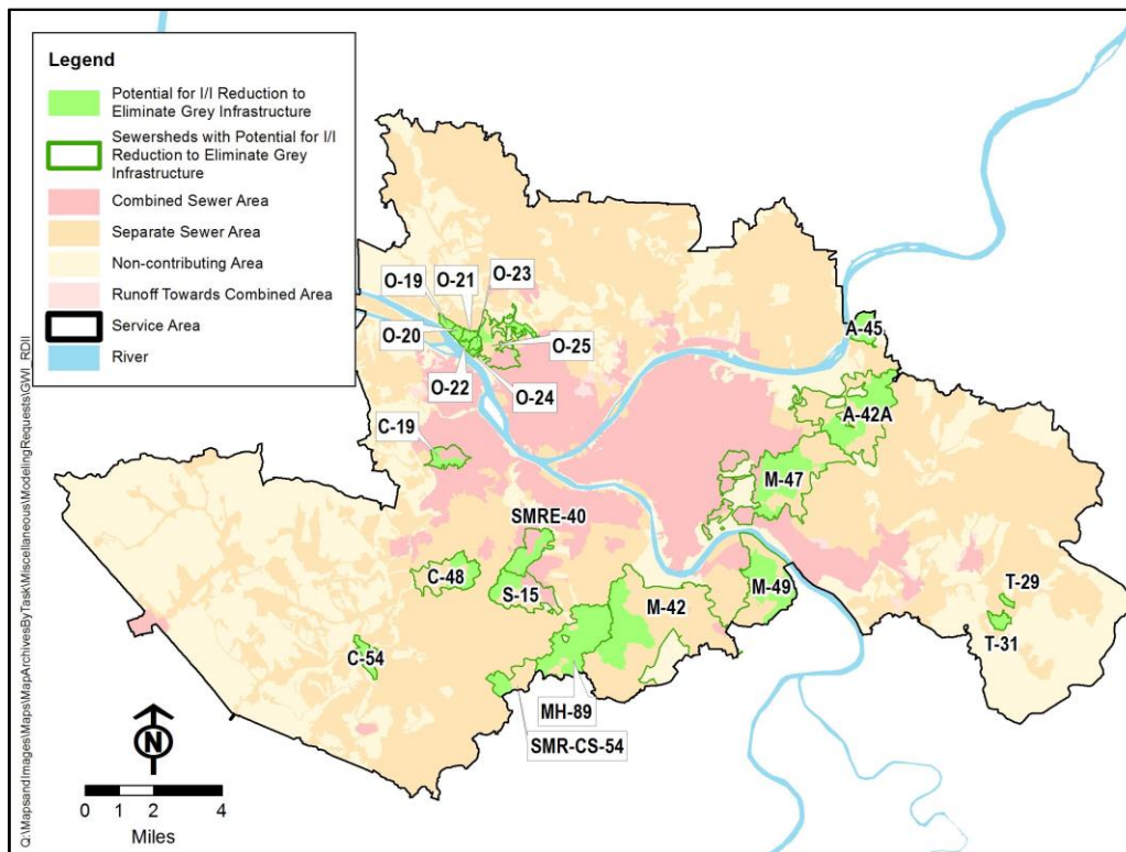
Figure 10-32: Location of Point of Connection Sewersheds with Greatest Potentials for I/I Reduction to Eliminate SSOs for 2-Year Design Storm
