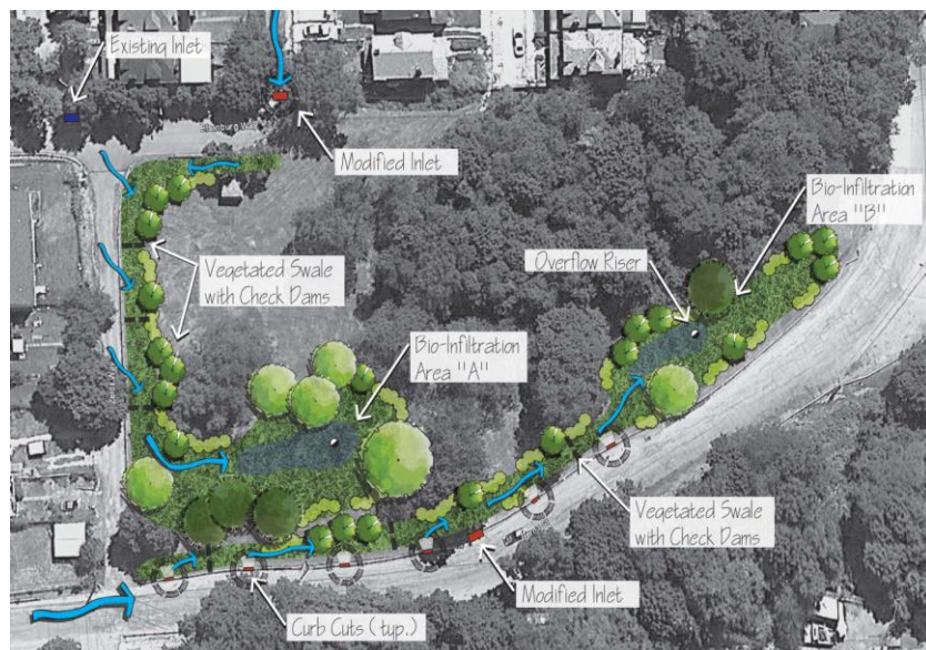
Figure 10-53: McKinley Park Bernd Street GSI Concept Layout
