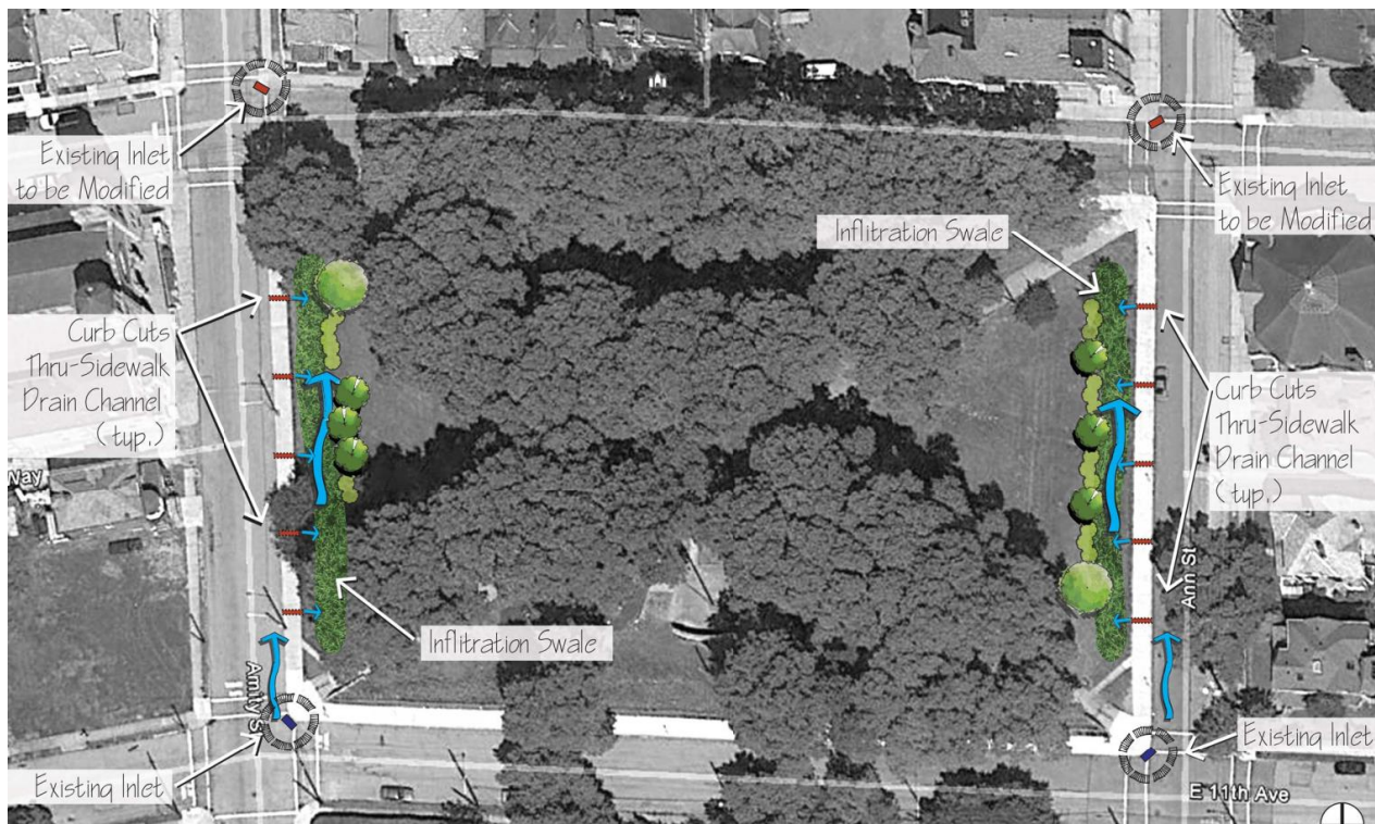
Figure 10-51: Homestead Borough GSI Concept Layout
