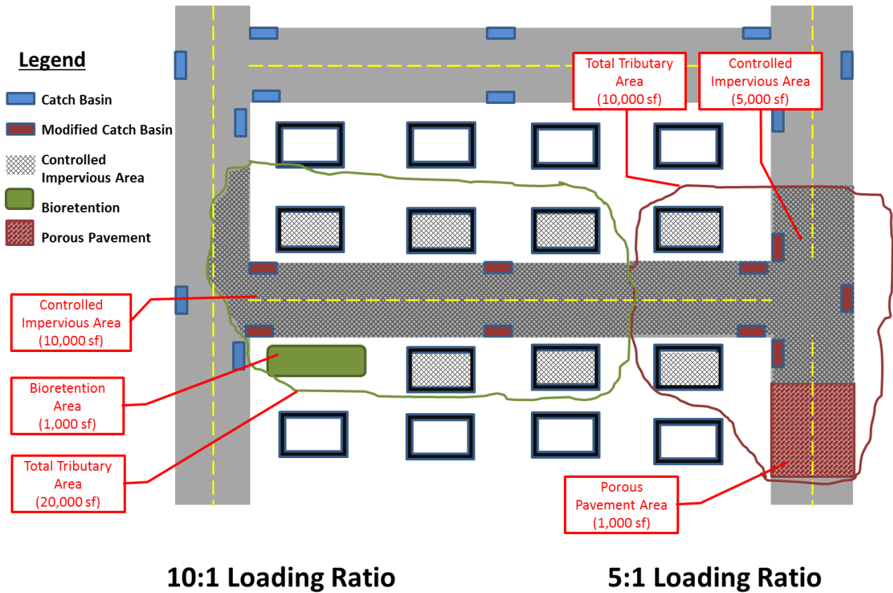
Figure 10-7: Illustration of Loading Ratio Definition
