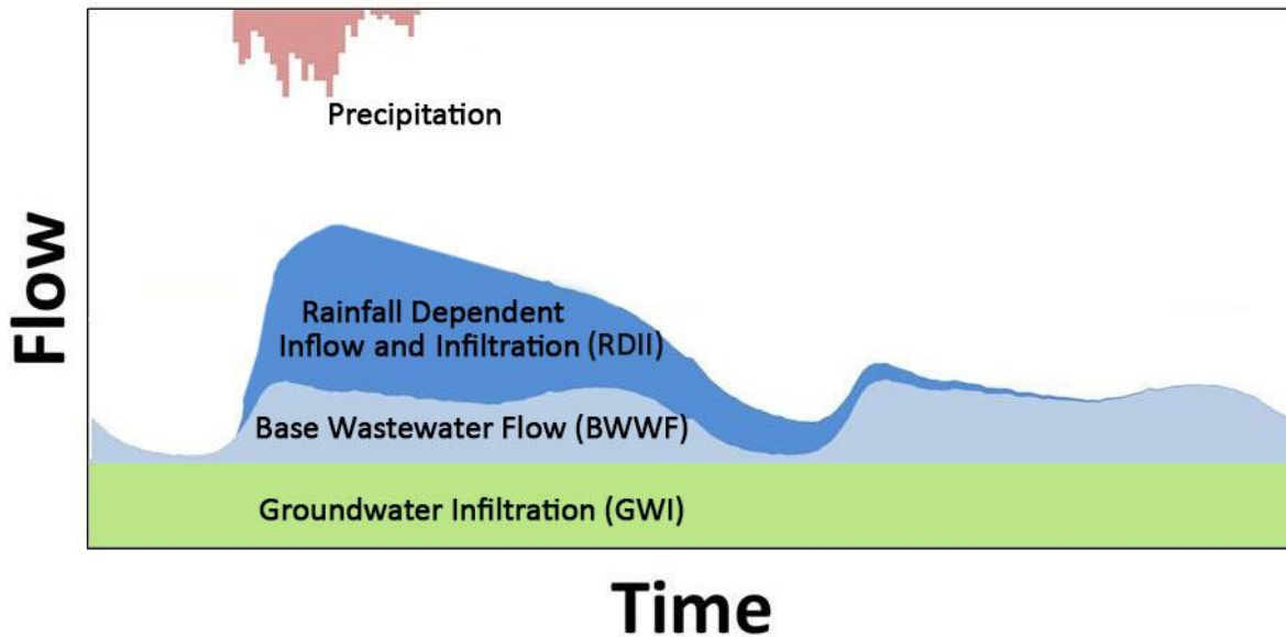
Figure 10-13: Three Components of Wastewater Flow in Separate Sanitary Sewer Systems
