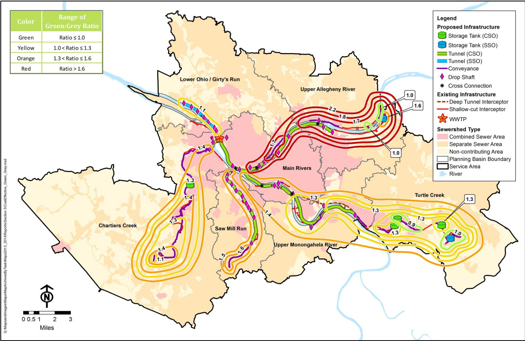
Figure 10-35: Summary of Downsizing Analysis “Loops” Depicting Portions of Downsizing Analysis with Selected Plan Cost Ratio Comparison Values
