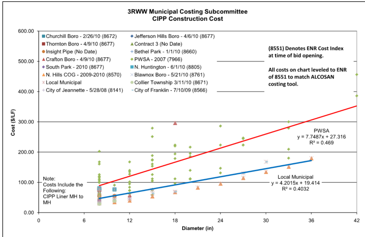
Figure 10-15: Data Plot of Local CIPP Construction Data
