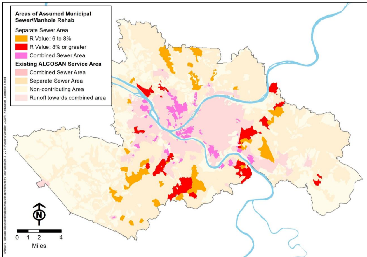
Figure 10-18: Sewer Rehabilitation Target Areas
