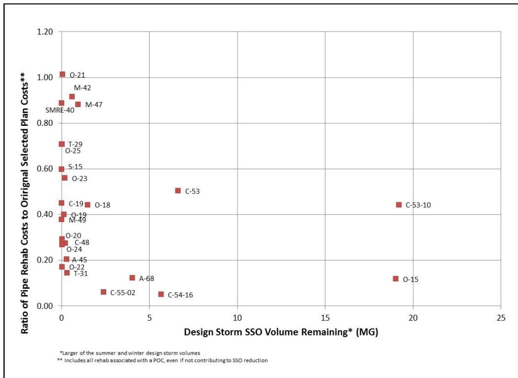
Figure 10-30: Potential of I/I Reduction to Eliminate SSOs – Point of Connection Sewersheds – Cost Ratio of One or Less
