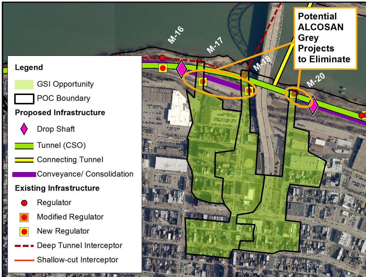
Figure 10-27: Example of Evaluating Opportunities to Eliminate Grey Projects with GSI for Outfalls M-17, M-18 and M-20
