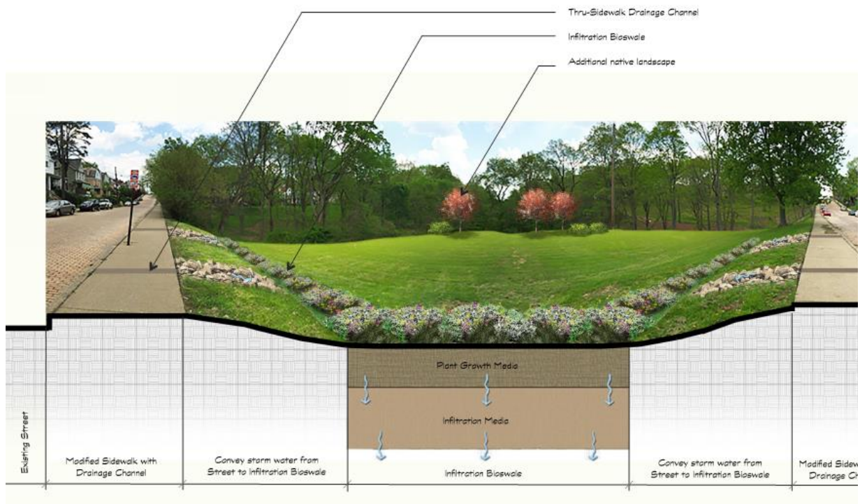
Figure 10-54: McKinley Park, Michigan Street GSI Concept Rendering
