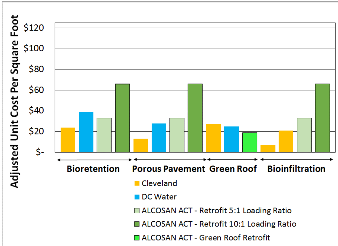
Figure 10-11: National Comparison – Capital Cost ($ per Square Foot) of Installed GSI
