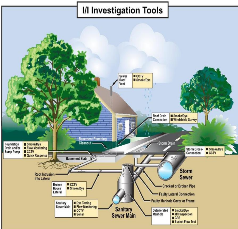
Figure 10-3: Pathways of Infiltration and Inflow (I/I) into Sanitary Sewer Systems and Various I/I Investigation Tools
