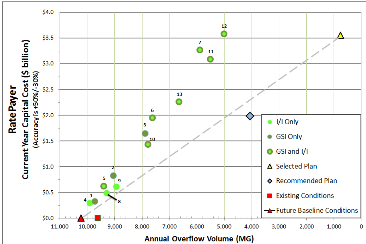
Figure 10-22: Capital Cost and Overflow Reduction without Redevelopment
