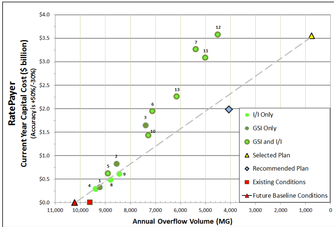
Figure 10-23: Capital Cost and Overflow Reduction with Redevelopment
