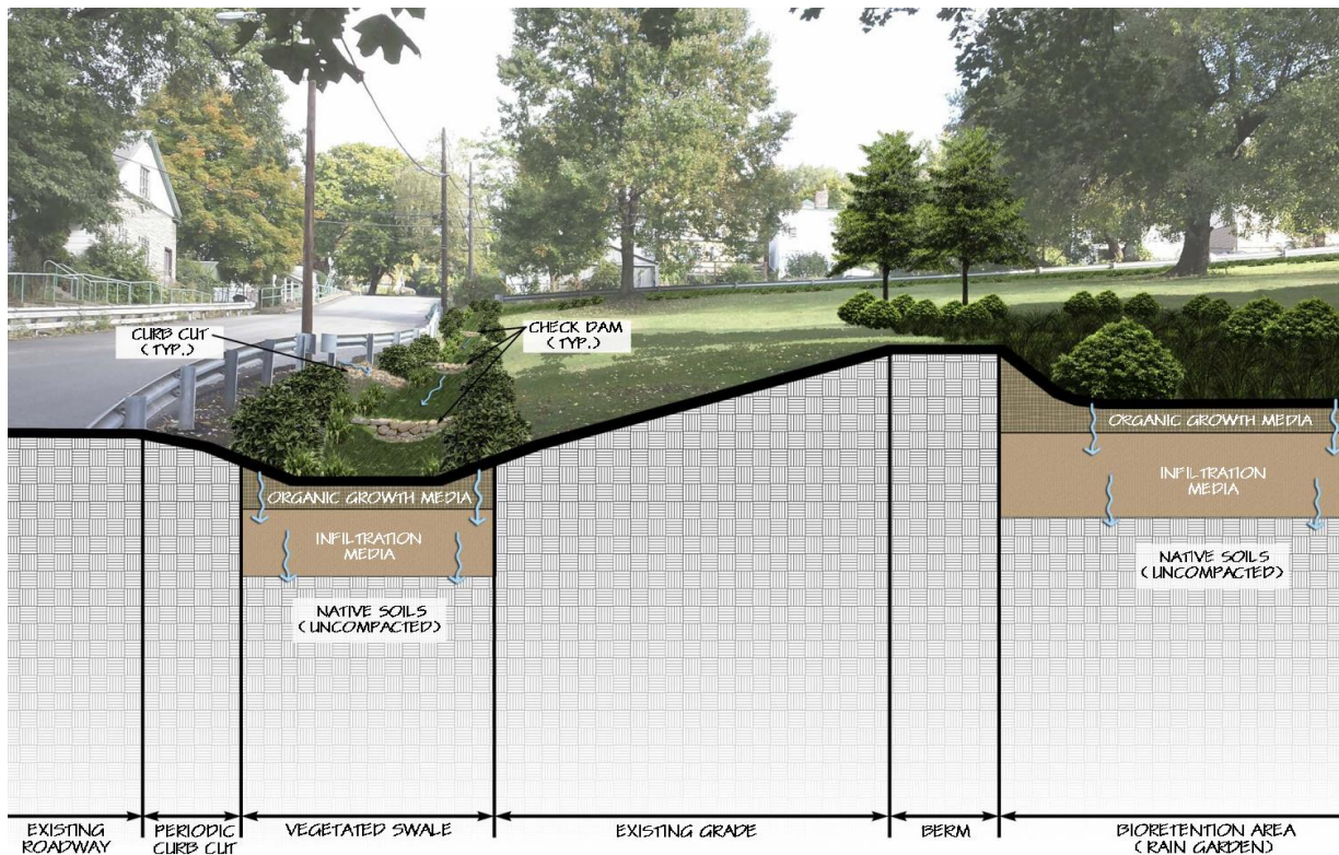
Figure 10-55: McKinley Park Rendering
