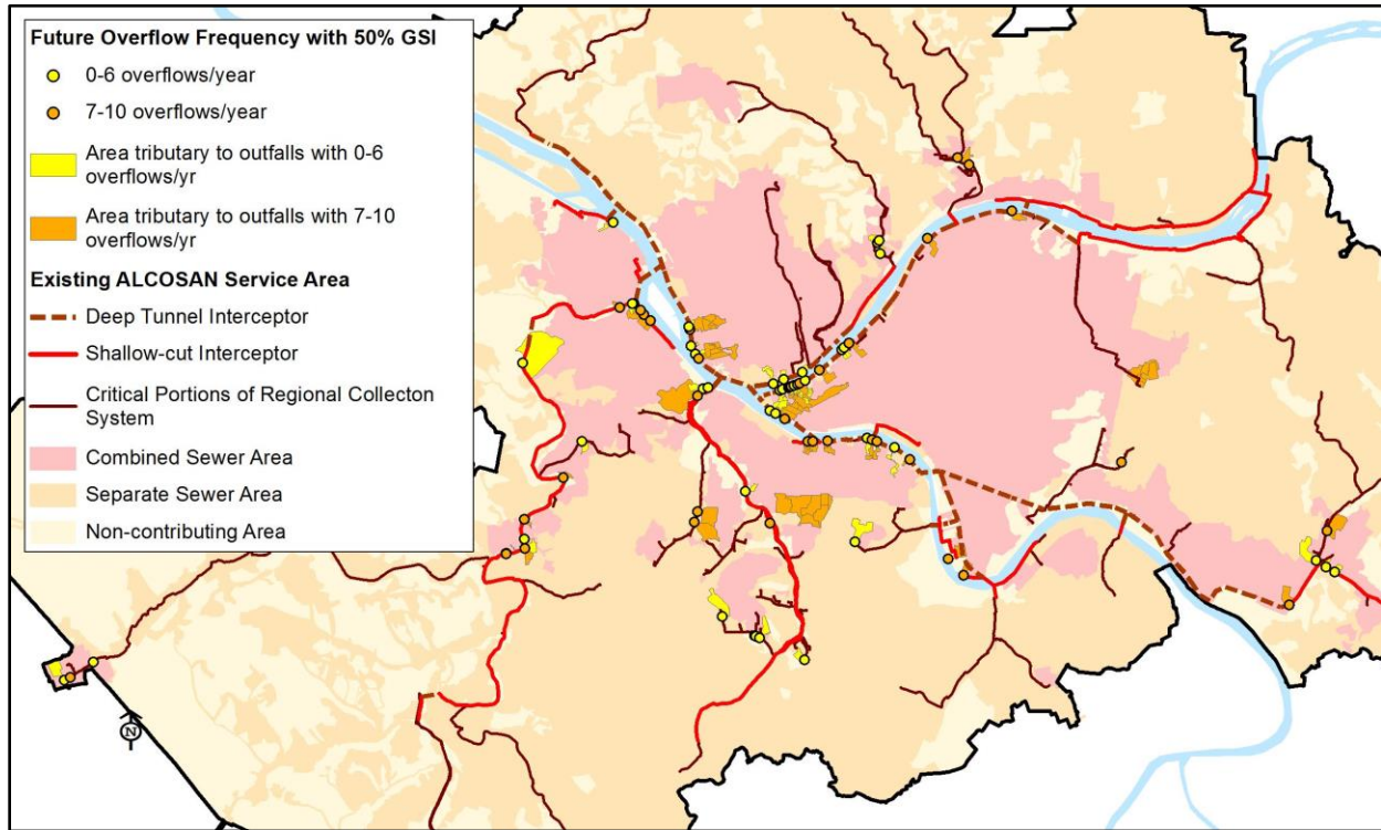
Figure 10-26: Outfalls in various Overflow Frequency ranges for the GSI only Alternative
